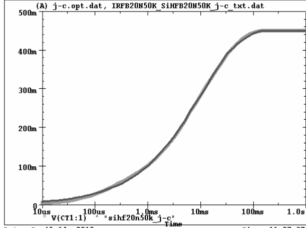
SiHFB20N50K Tank j-c Temperature: 27.0
