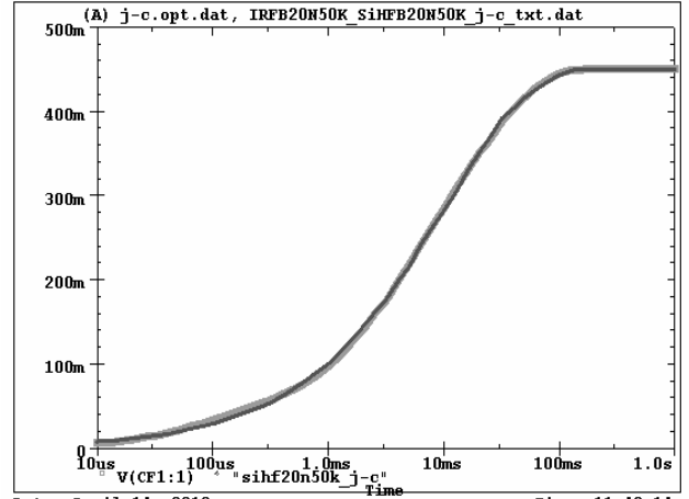
SiHFB20N50K Filter j-c Temperature: 27.0
